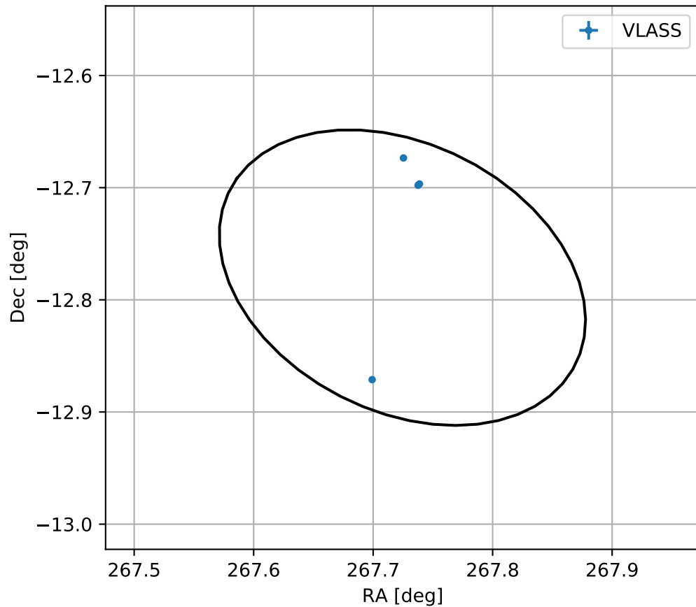
4FGL J1750.8-1246
