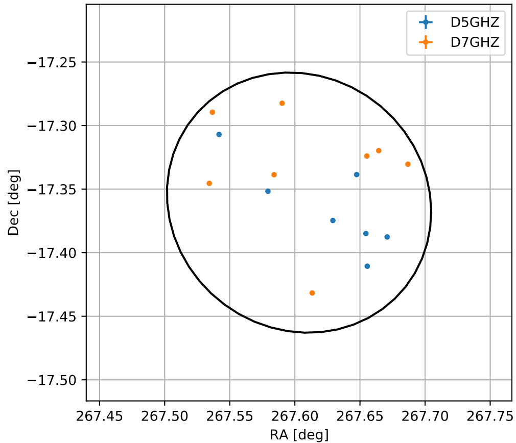
4FGL J1750.4-1721
