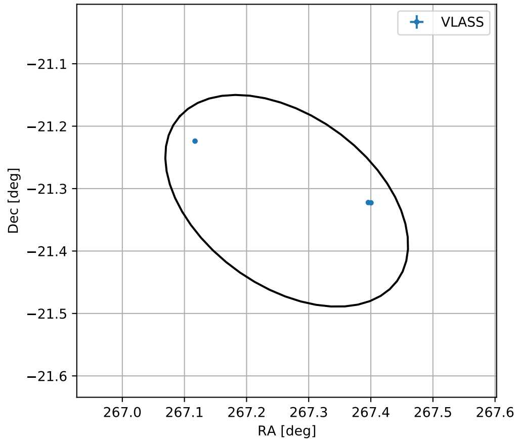
4FGL J1749.0-2119
