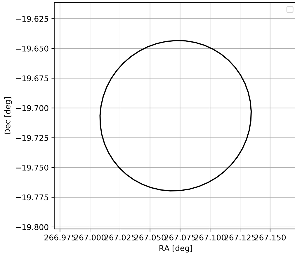
4FGL J1748.2-1942
