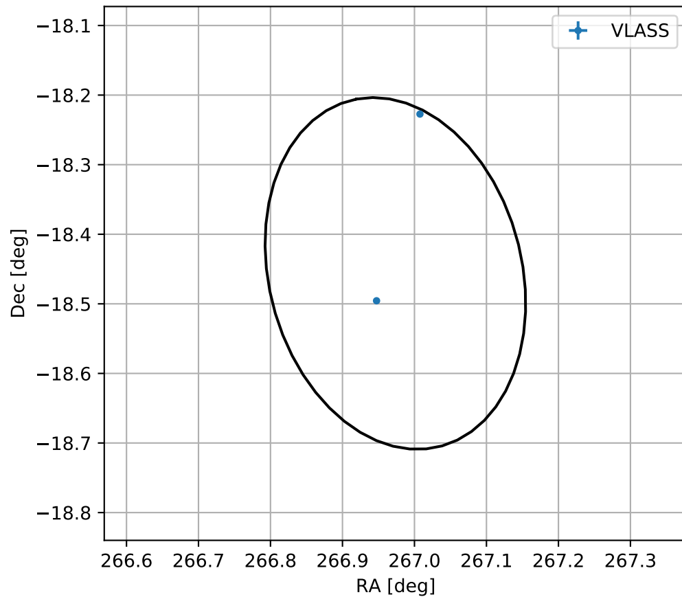
4FGL J1747.8-1827
