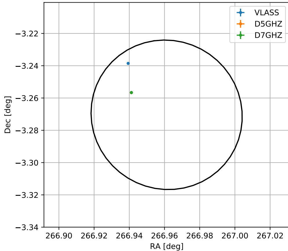
4FGL J1747.8-0316
