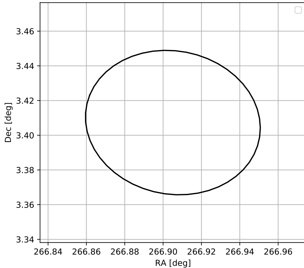
4FGL J1747.6+0324
