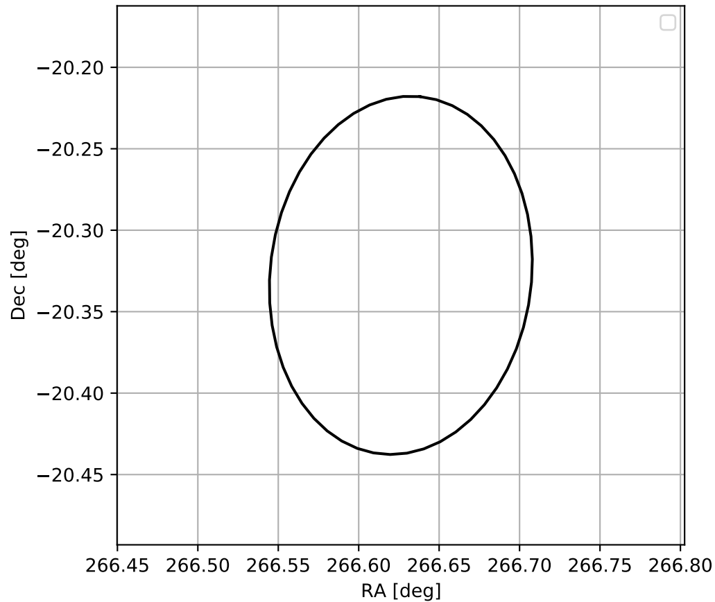
4FGL J1746.5-2019
