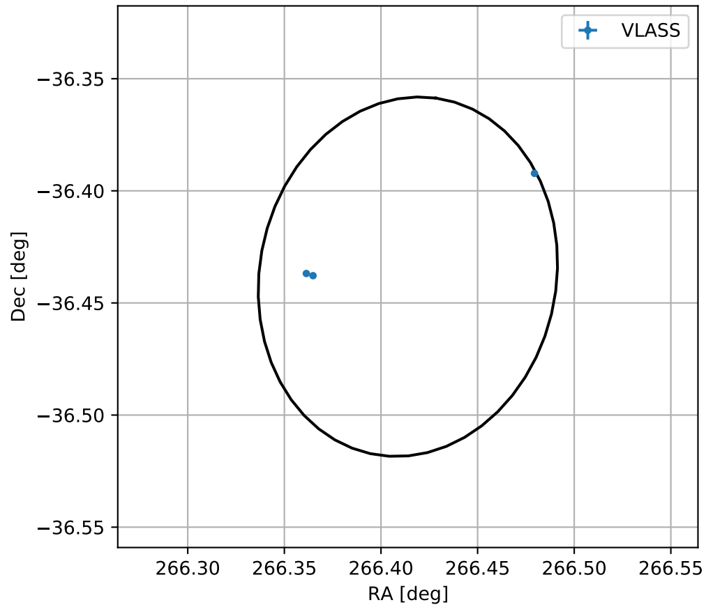
4FGL J1745.6-3626
