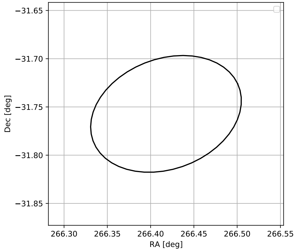
4FGL J1745.6-3145
