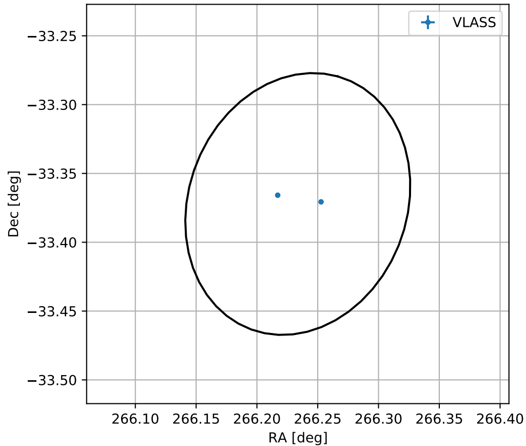
4FGL J1744.9-3322
