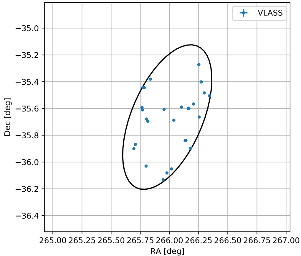
4FGL J1743.9-3539
