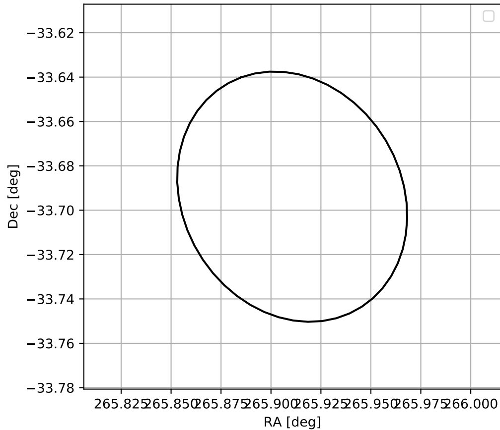
4FGL J1743.6-3341
