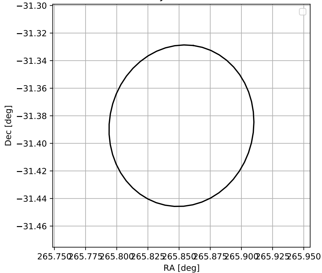
4FGL J1743.4-3123
