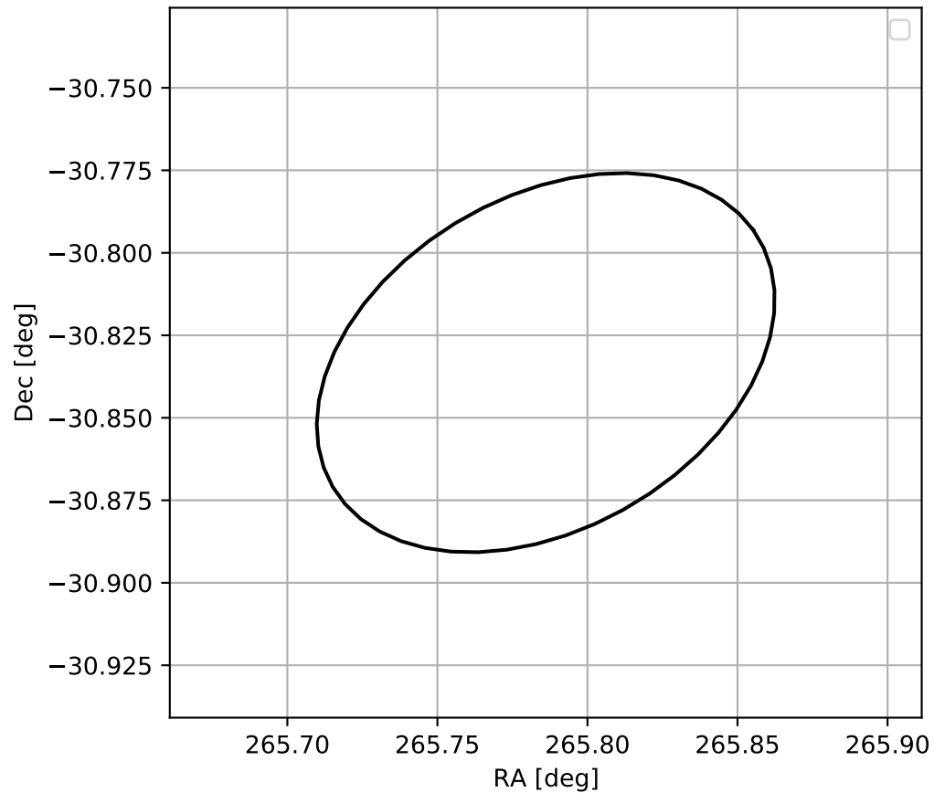
4FGL J1743.1-3049c
