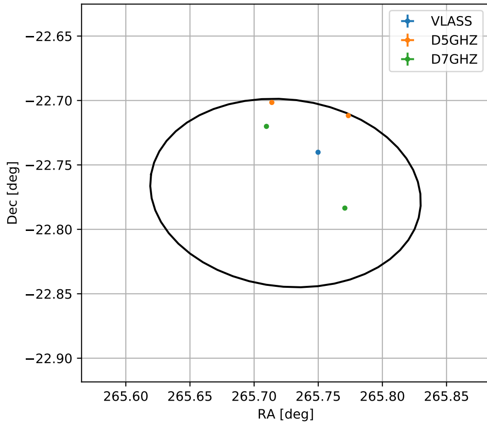
4FGL J1742.8-2246
