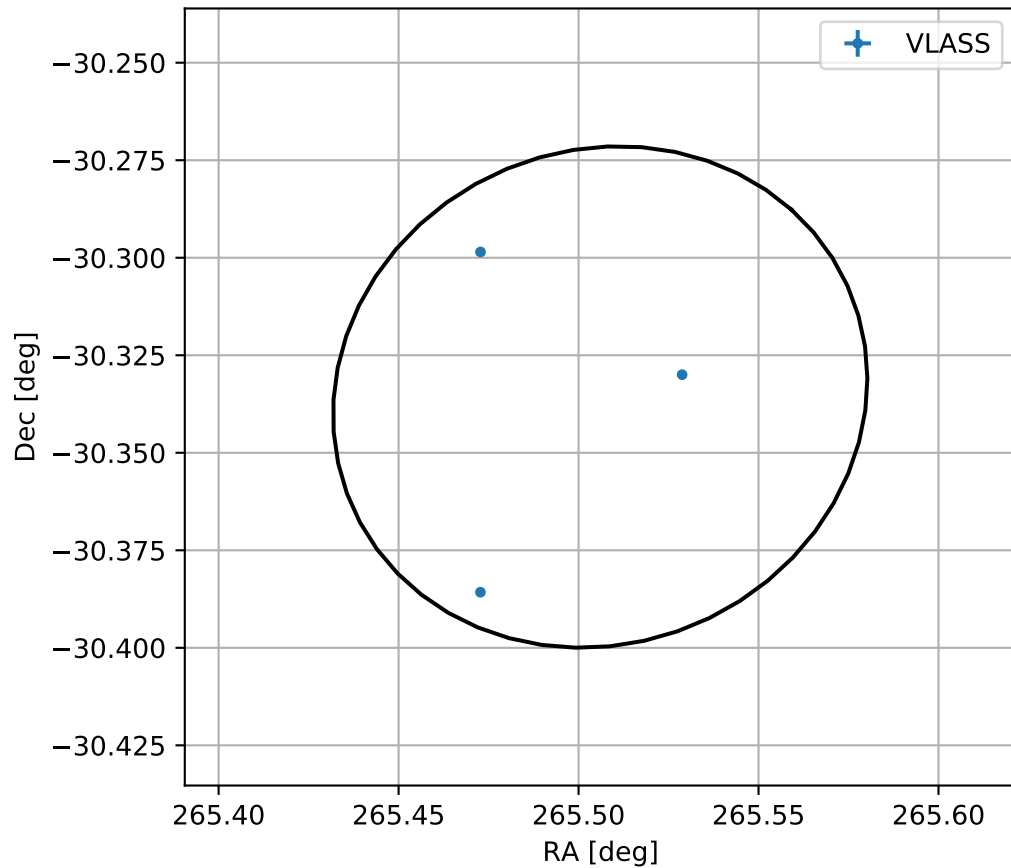
4FGL J1742.0-3020
