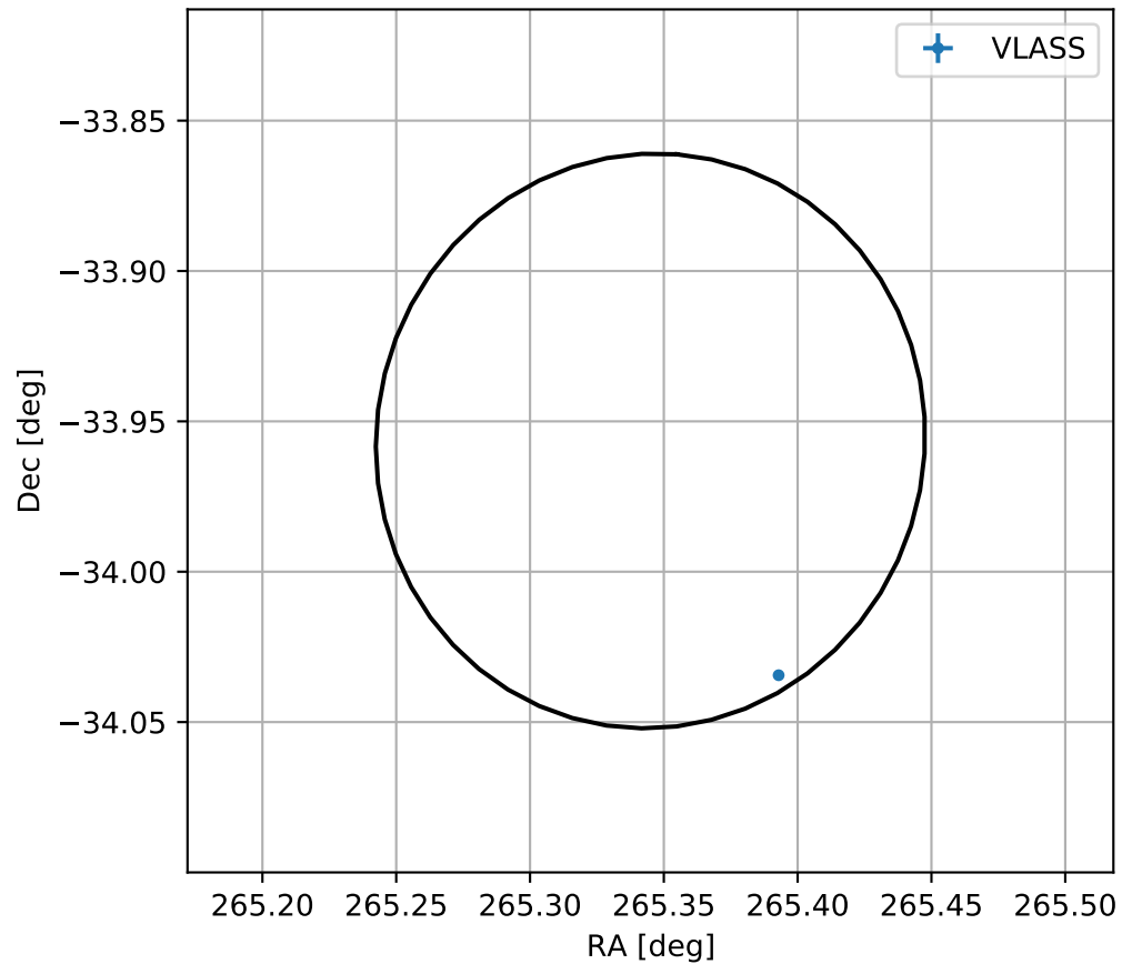
4FGL J1741.3-3357
