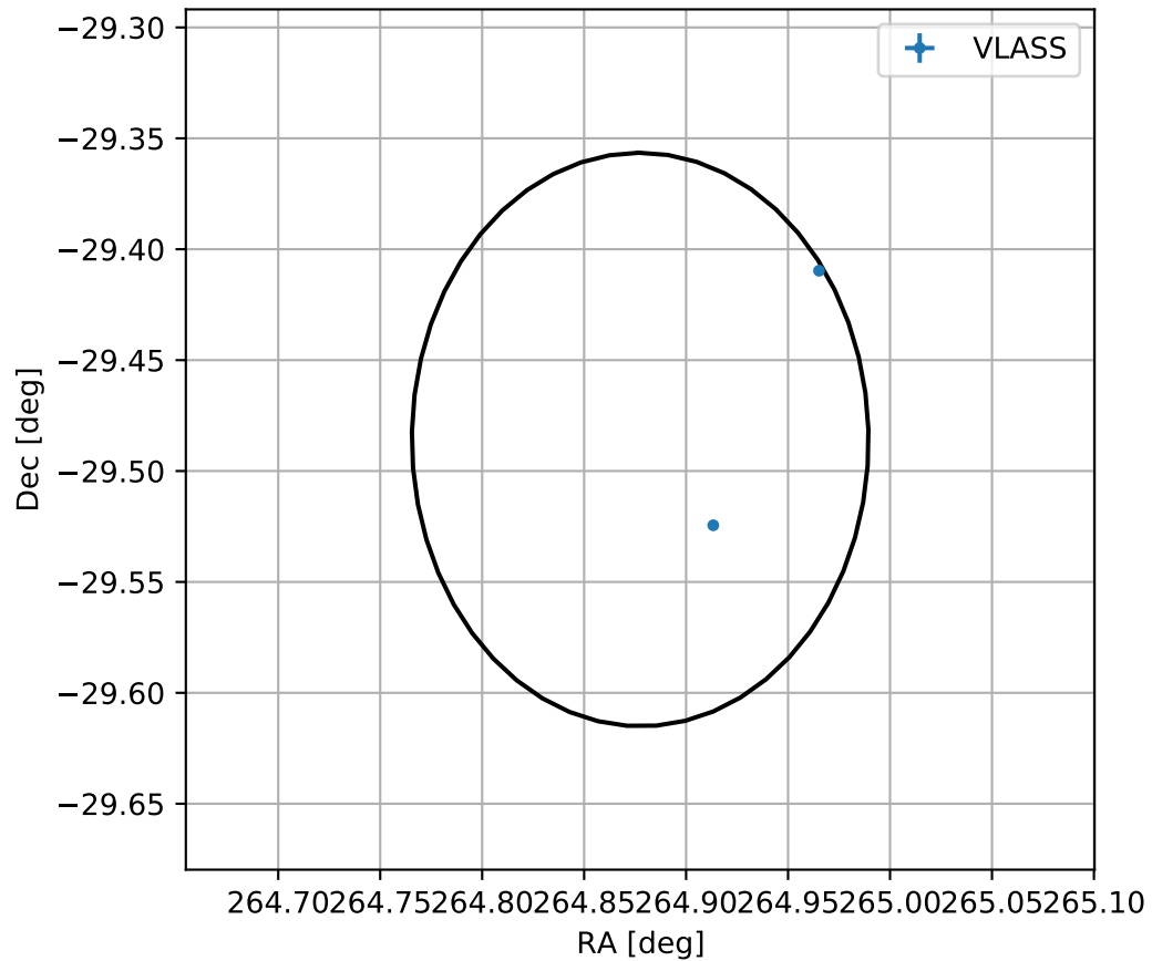
4FGL J1739.5-2929
