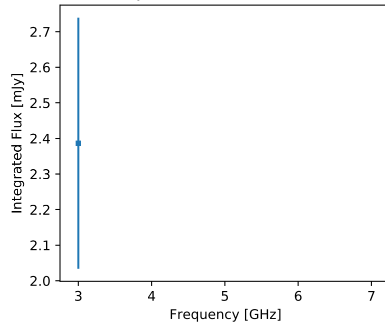
F357 J173928.23-253111.9 (unr)
