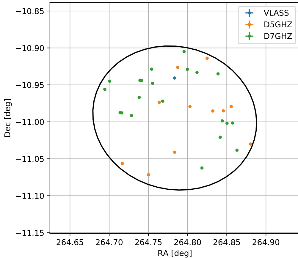
4FGL J1739.1-1059
