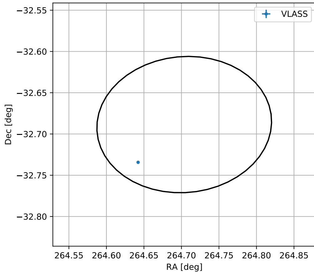
4FGL J1738.8-3241
