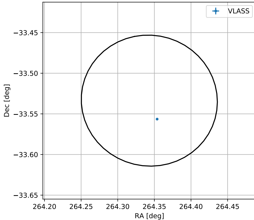
4FGL J1737.3-3332
