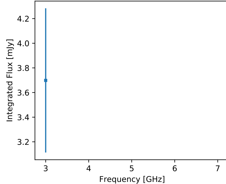
F357 J173724.90-333323.2 (unr)
