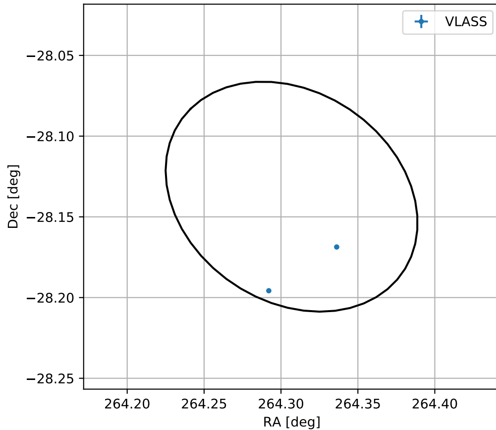
4FGL J1737.2-2808
