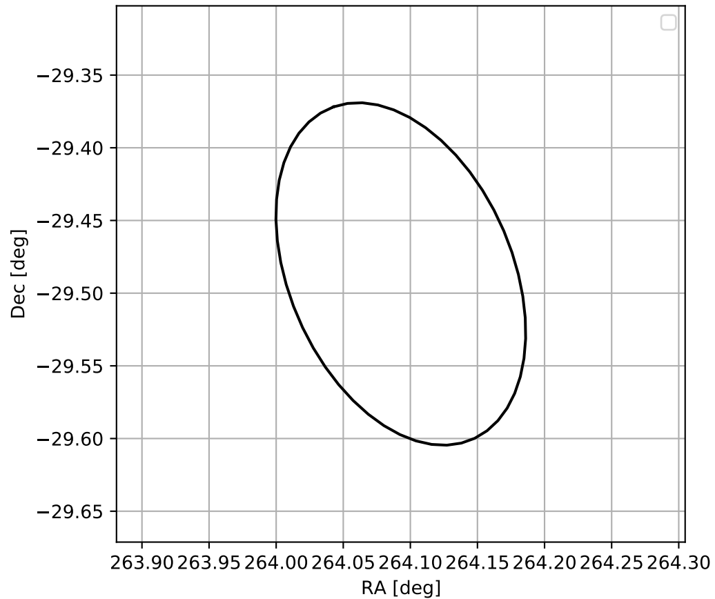
4FGL J1736.3-2929
