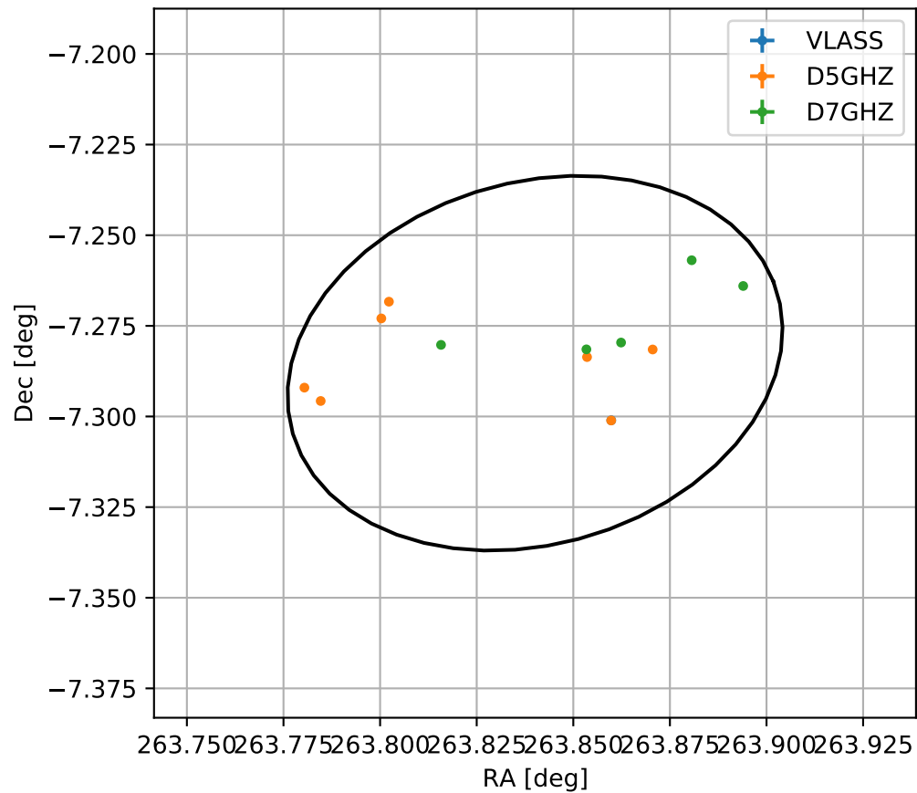
4FGL J1735.3-0717
