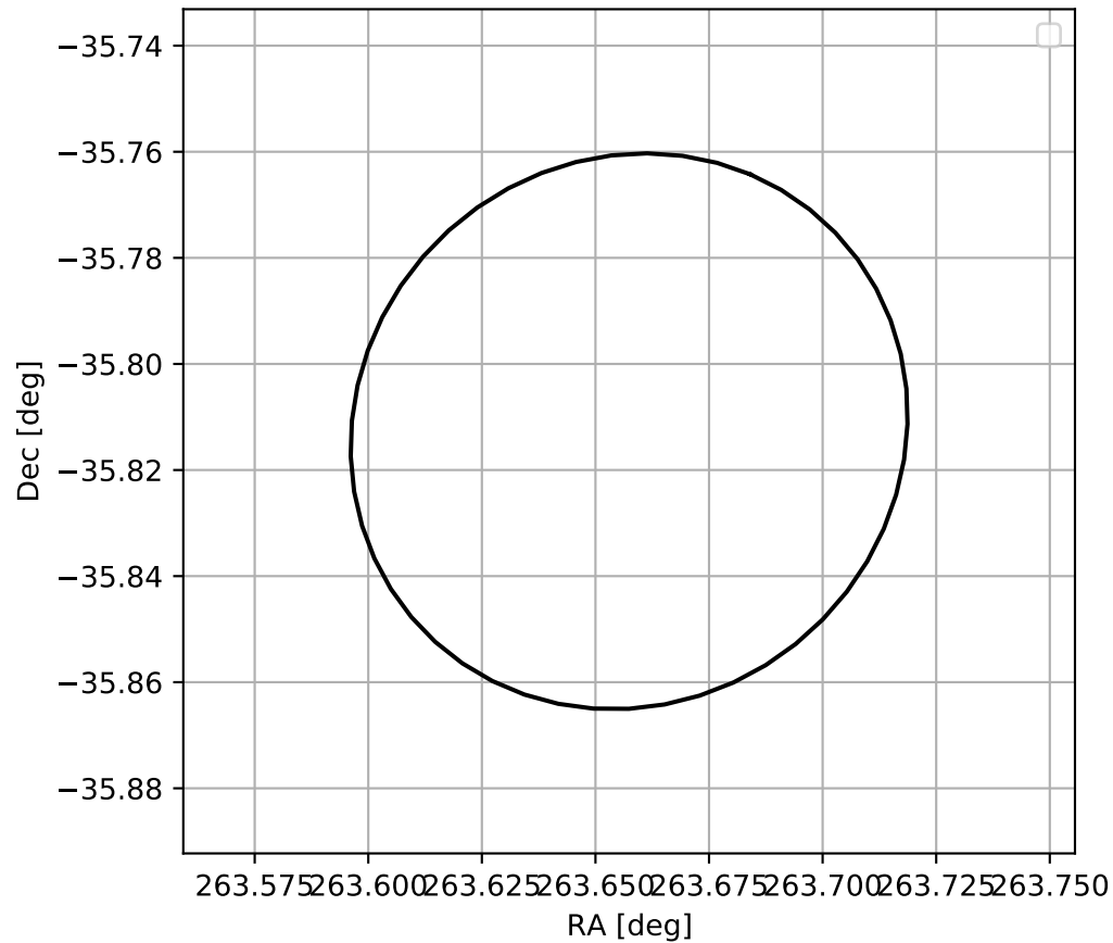
4FGL J1734.6-3548
