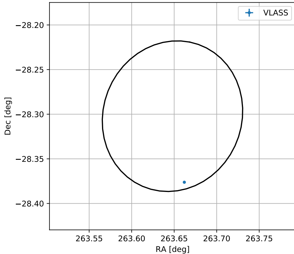
4FGL J1734.5-2818
