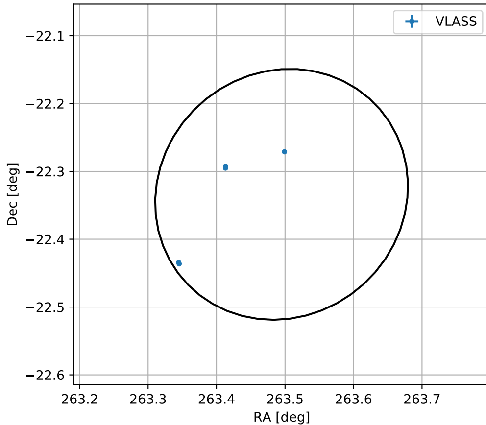
4FGL J1733.9-2220
