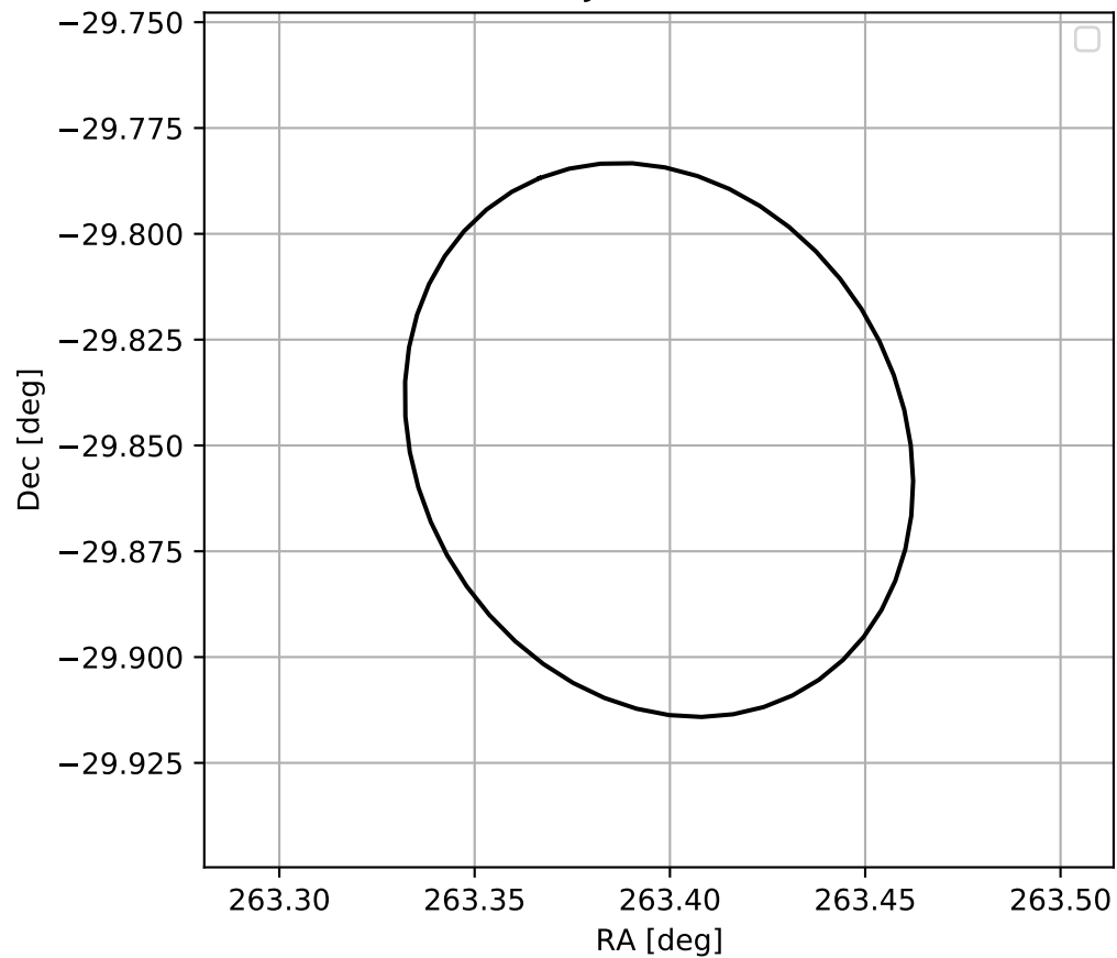
4FGL J1733.5-2950
