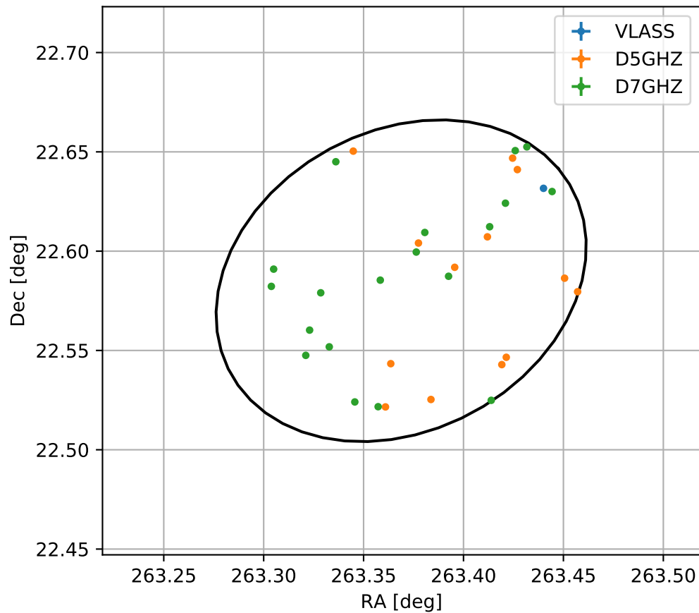
4FGL J1733.4+2235
