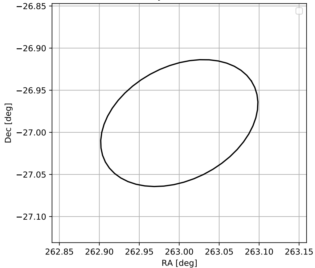
4FGL J1732.0-2659
