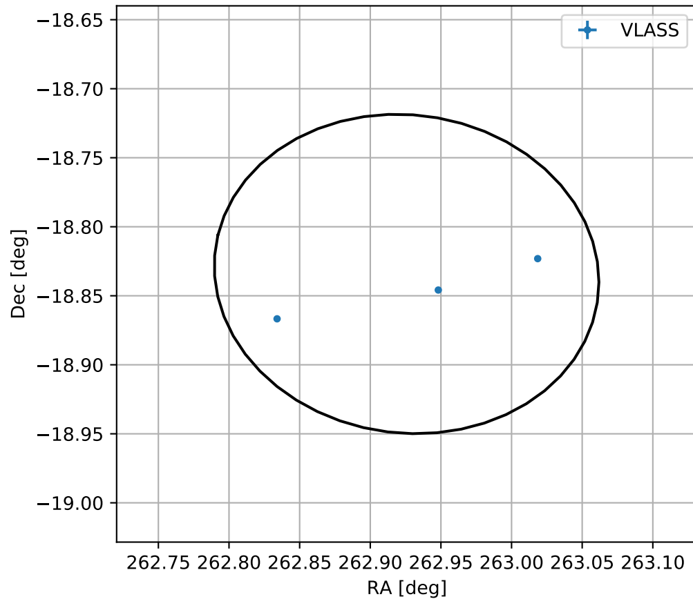
4FGL J1731.7-1850
