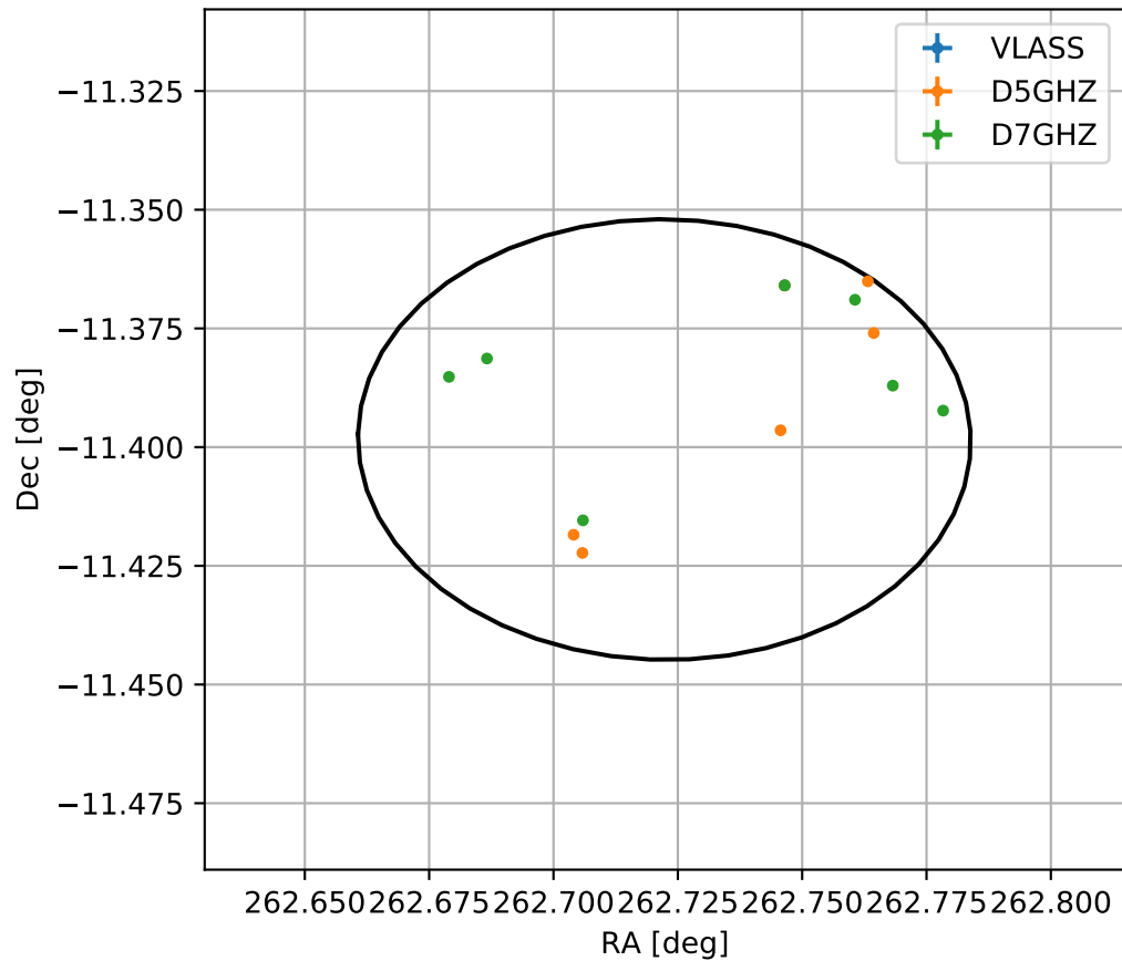
4FGL J1730.8-1123
