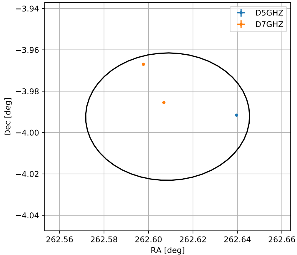
4FGL J1730.4-0359
