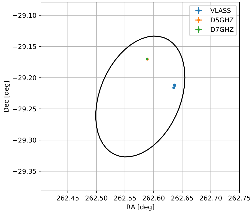
4FGL J1730.3-2913
