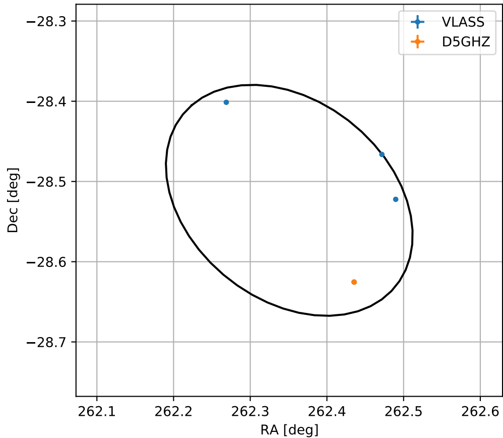
4FGL J1729.4-2831
