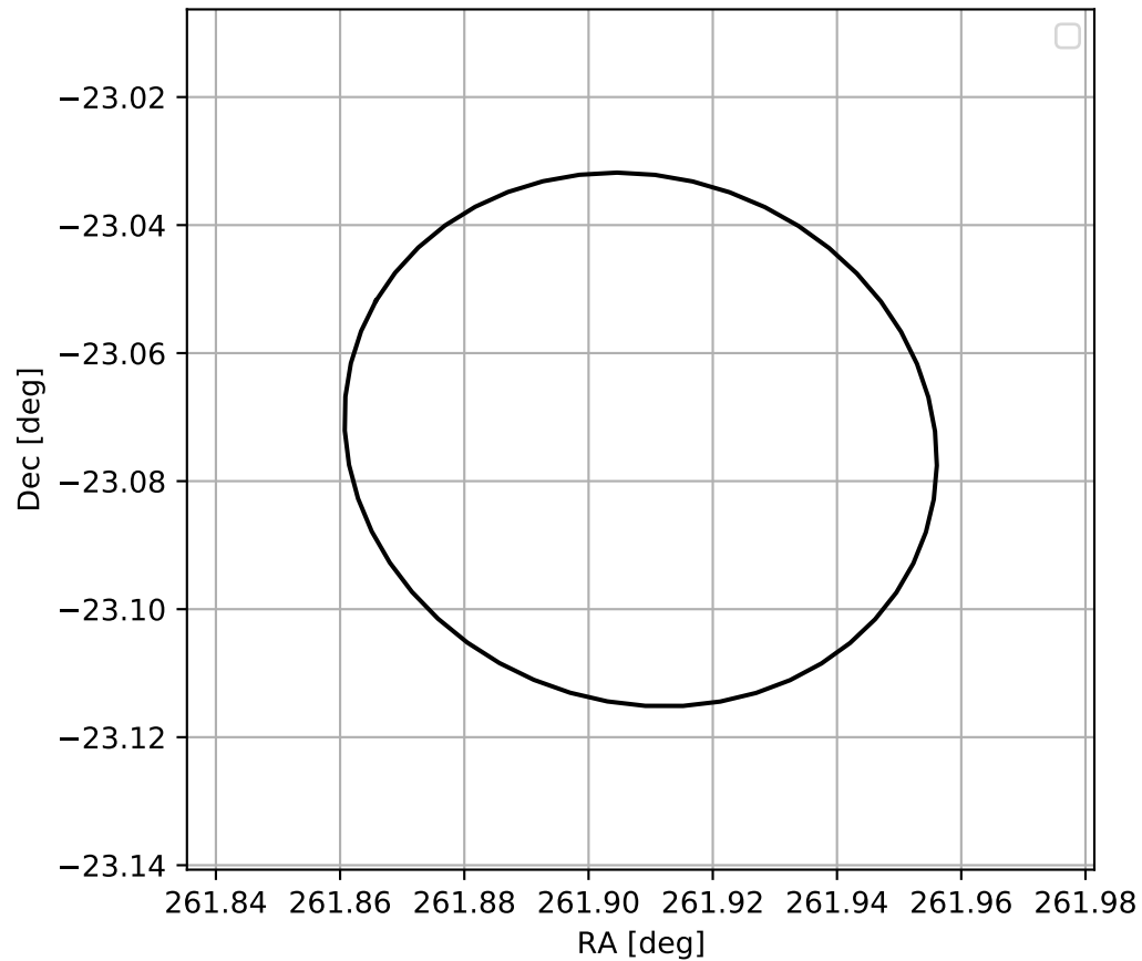
4FGL J1727.6-2304
