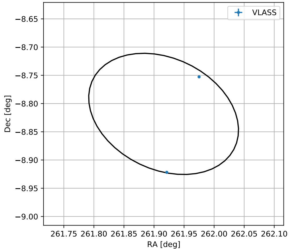
4FGL J1727.6-0849
