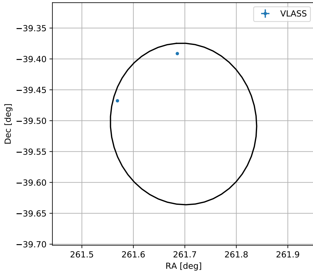
4FGL J1726.7-3930
