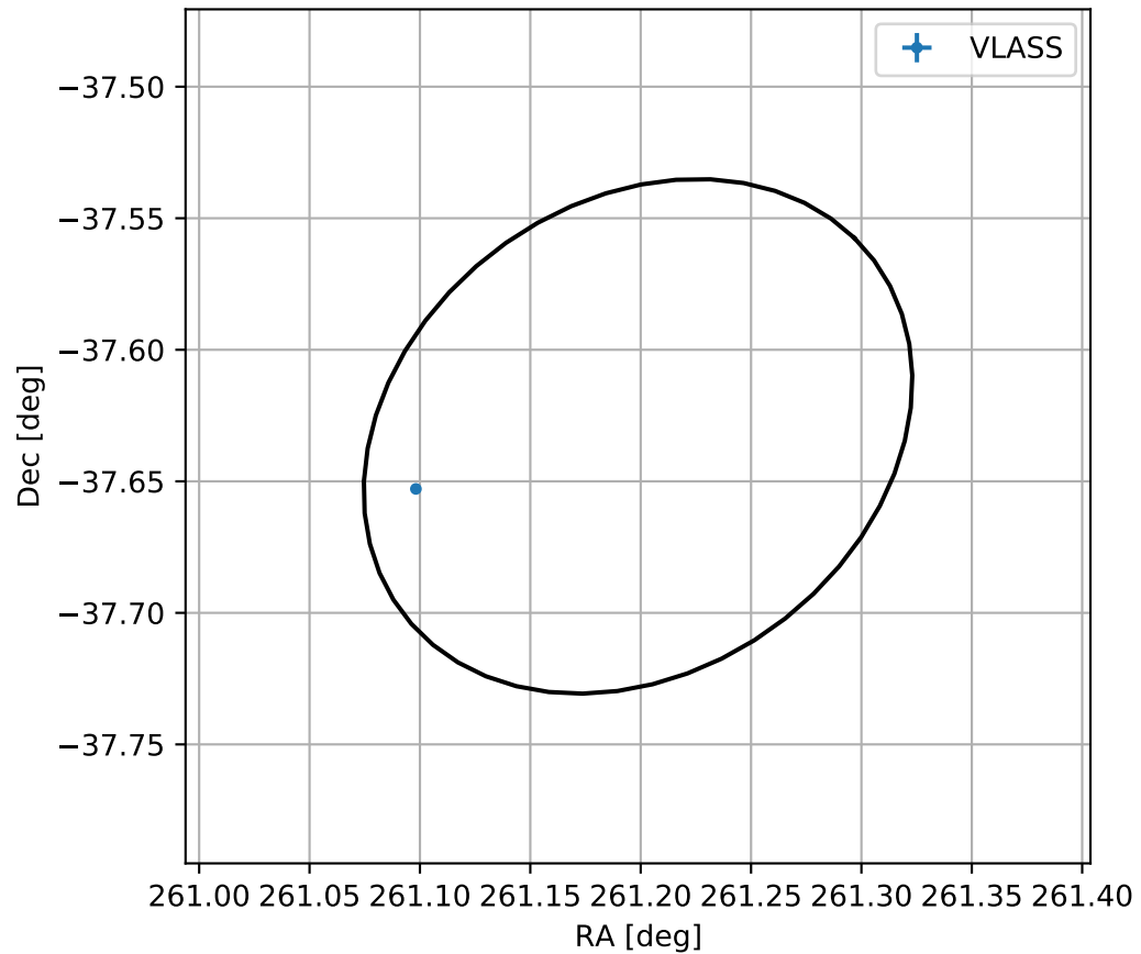
4FGL J1724.7-3737
