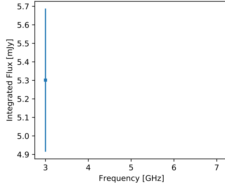
F357 J172423.56-373910.3 (unr)
