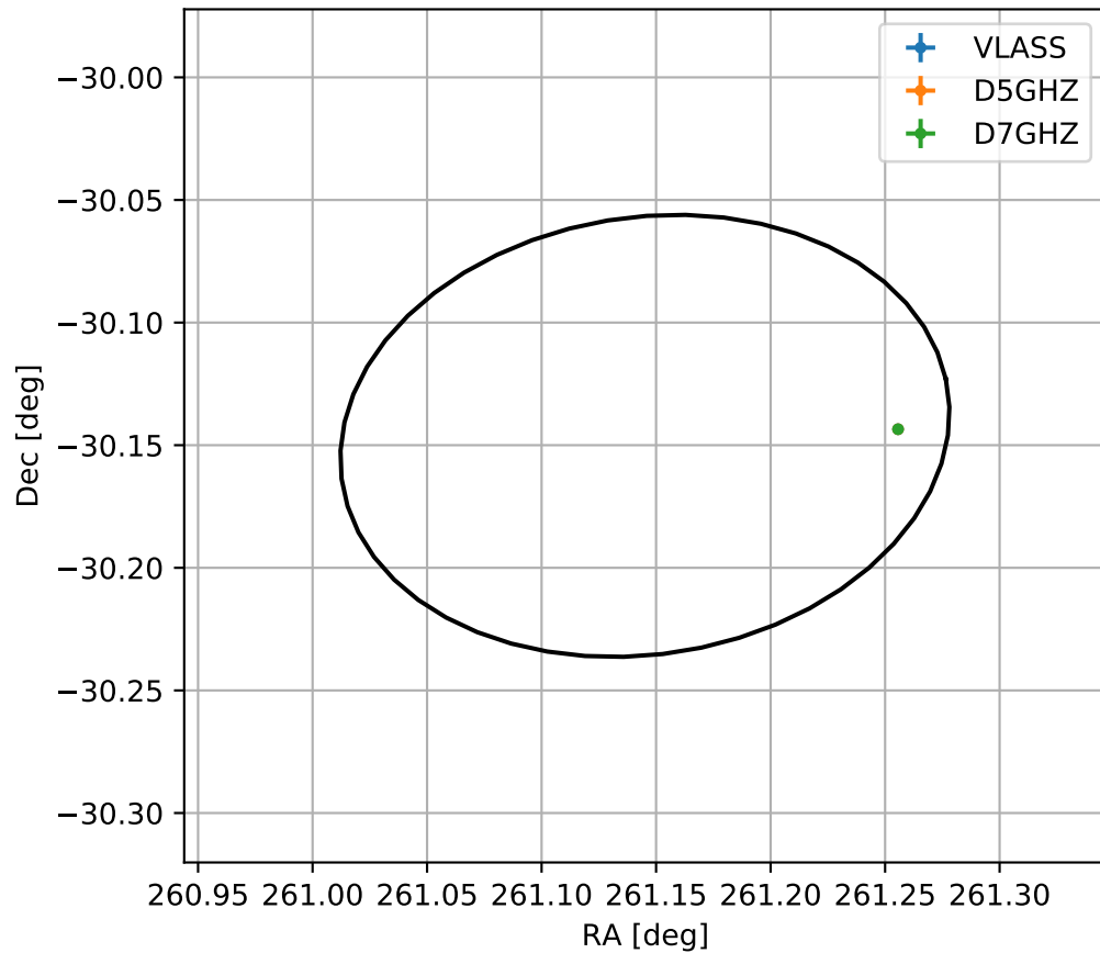
4FGL J1724.5-3008
