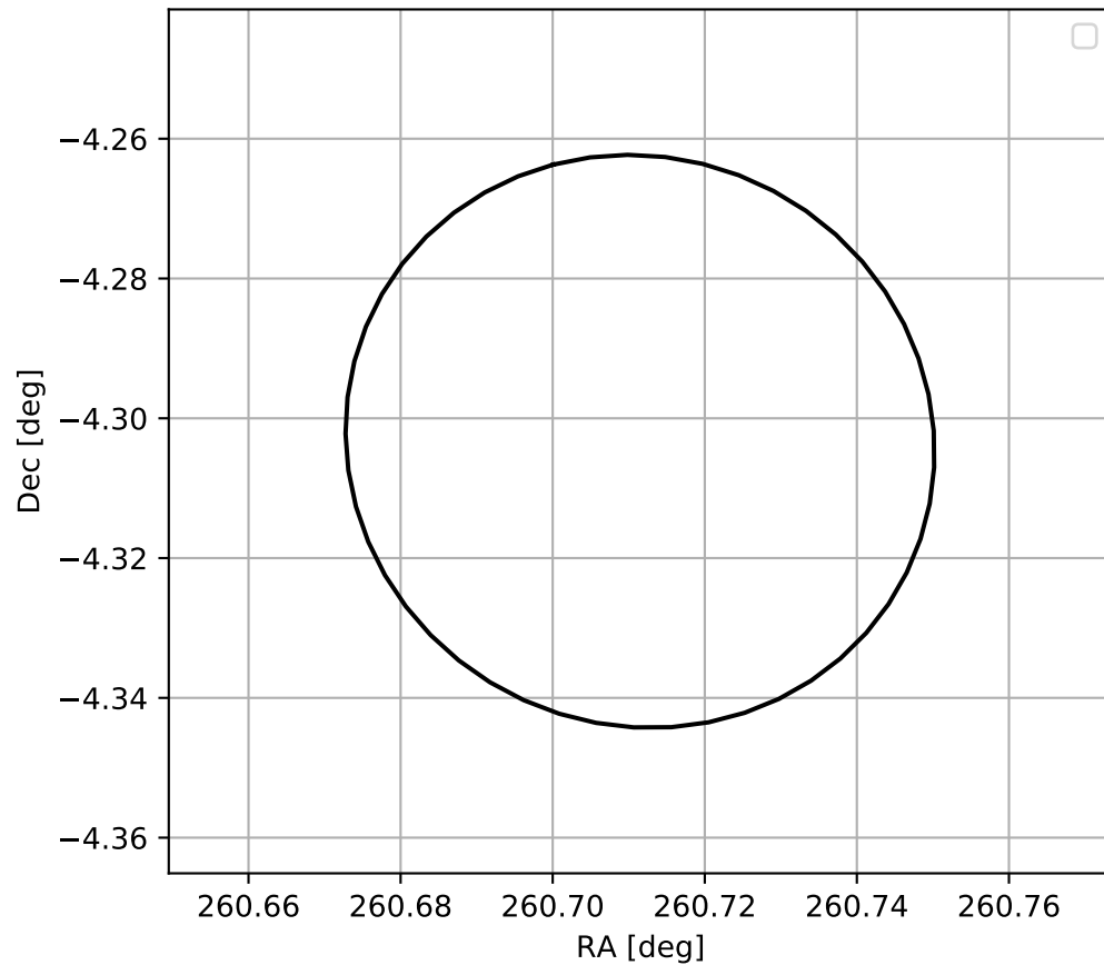
4FGL J1722.8-0418
