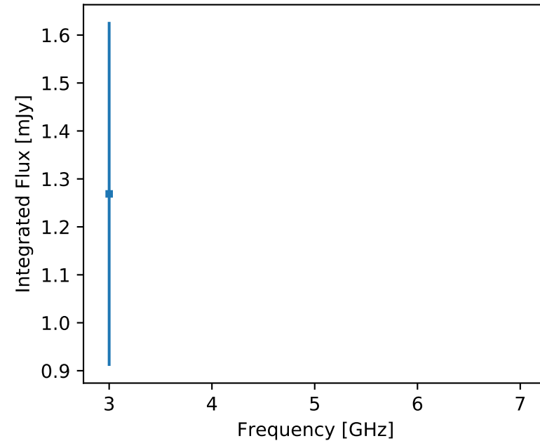
F357 J172202.96-320744.8 (unr)
