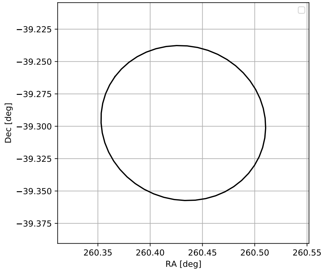
4FGL J1721.7-3917
