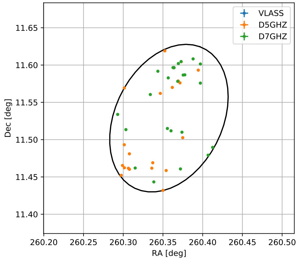
4FGL J1721.4+1131
