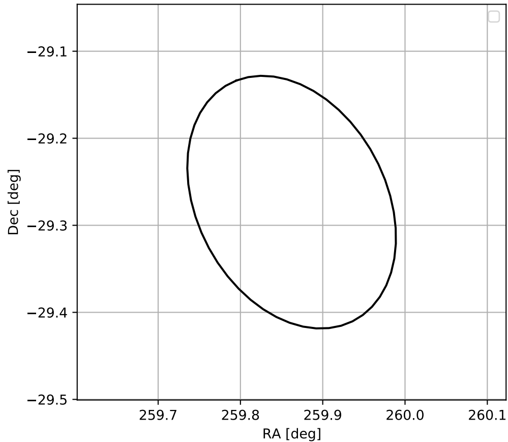
4FGL J1719.4-2916
