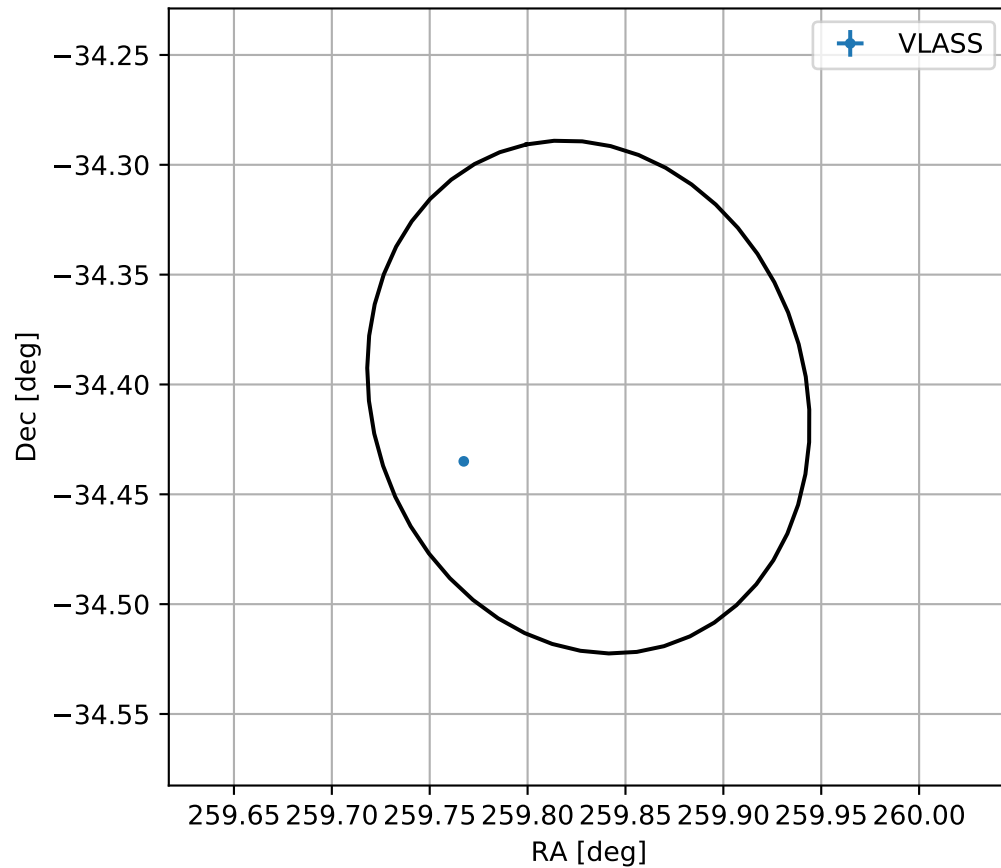
4FGL J1719.3-3424
